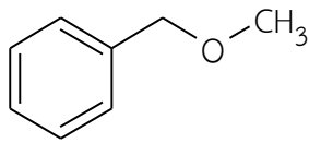
benzyl methyl ether
