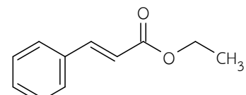
ethyl cinnamate (cinnamon)
