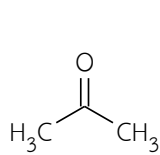
propanone (acetone)
