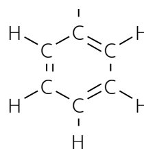
phenyl ( \text{C}_6\text{H}_5- )
