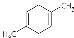
1,4-dimethylcyclohexa-1,4-diene
