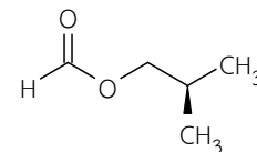
isobutyl formate (raspberry)
