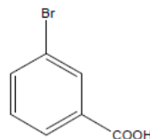
3-bromobenzoic acid
