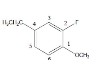
4-Ethyl-2-fluoroanisole
