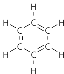
benzene ( \text{C}_6\text{H}_6 )
