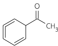
acetophenone (methyl phenyl ketone)
