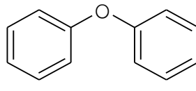
diphenyl ether
