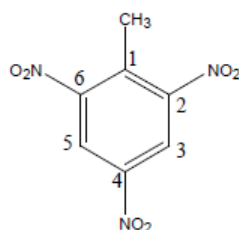
2,4,6-Trinitrotoluene
